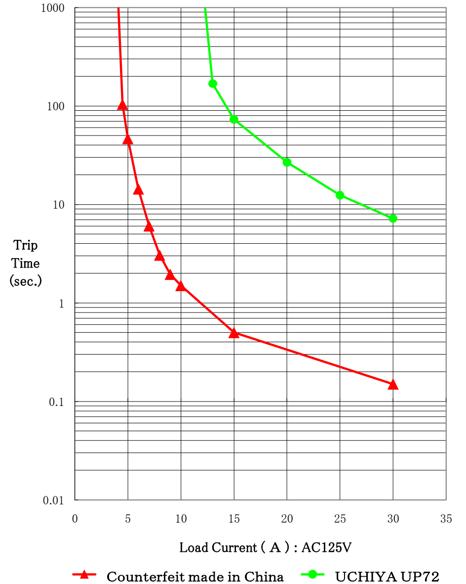
Trip Time against Load Current (Ampere) at 25°C
